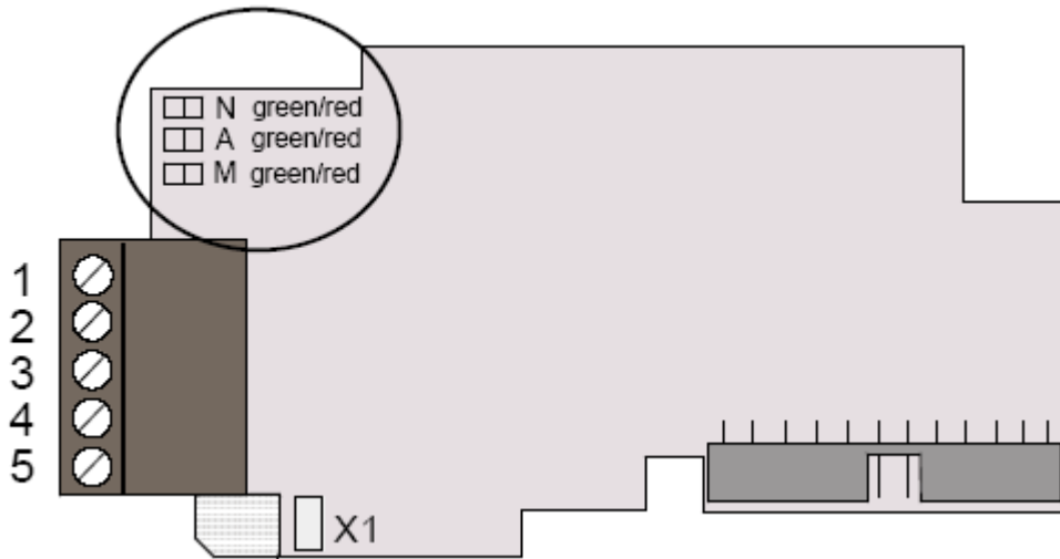
Figure 4-2. LED Indicators on the DeviceNet Board
