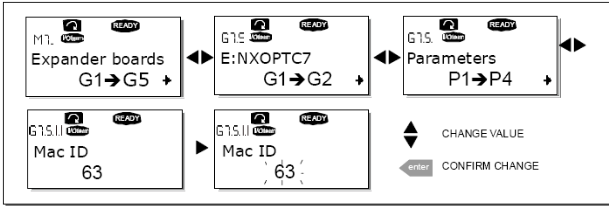
Figure 6-1. Changing the DeviceNet Board Parameter Values
