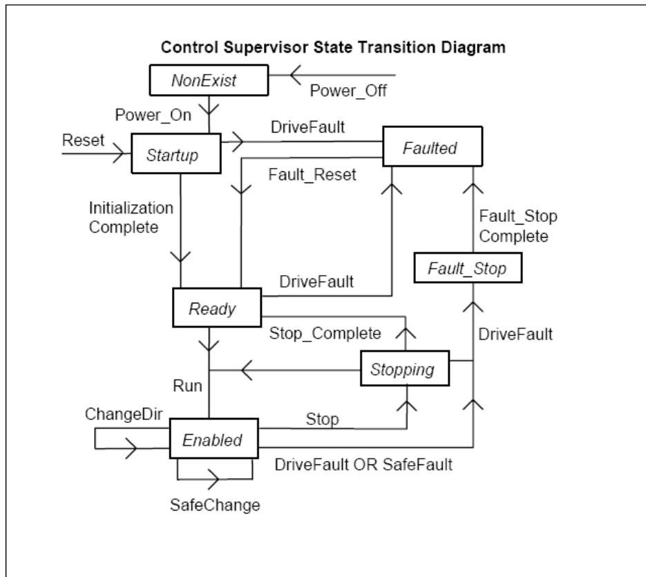
Figure 7-2. Control Supervisor State Transition Diagram
