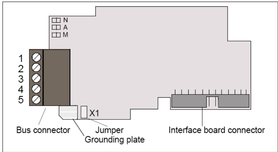
Figure 4-1. DeviceNet Option Board OPC7
